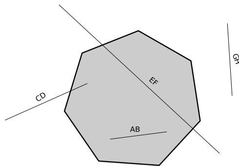
Figure 166: Example image used for line/polygon collision detection
